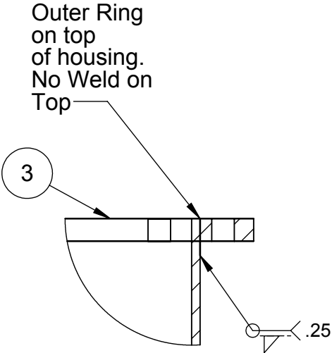
DETAIL J SCALE 1 : 3
