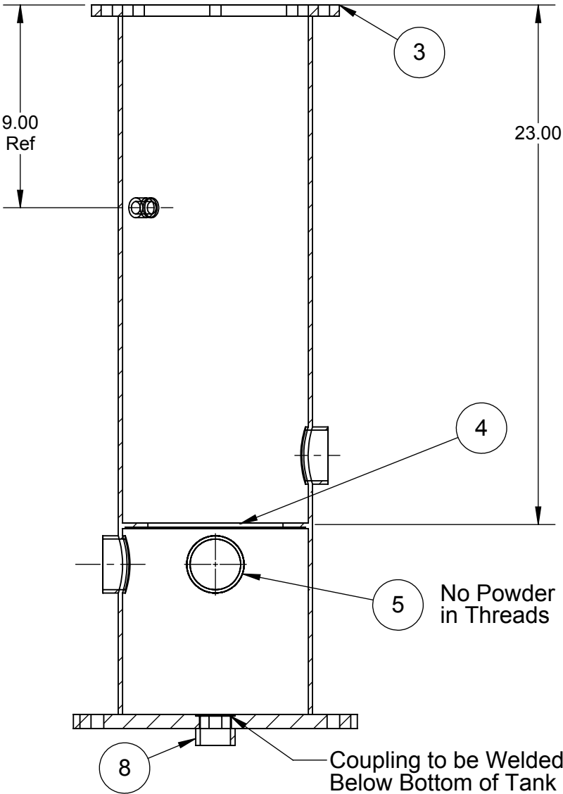
SECTION B-B
