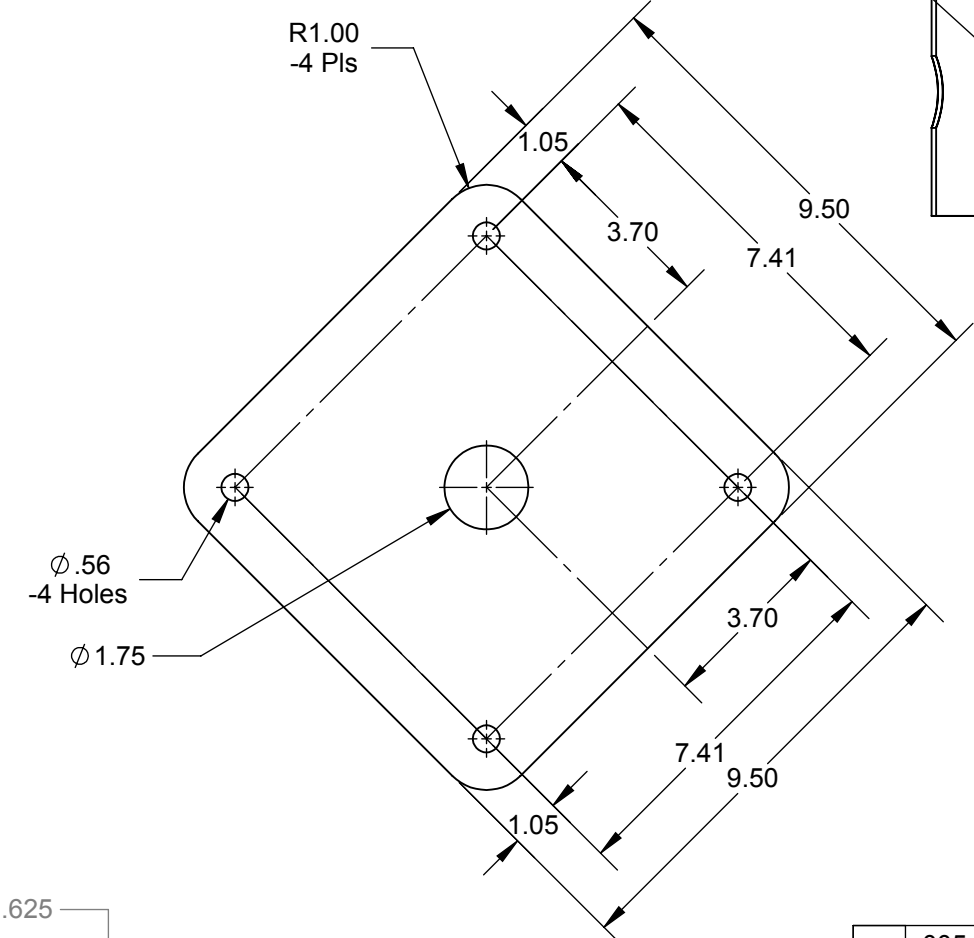
Bottom Base, A36 Steel
