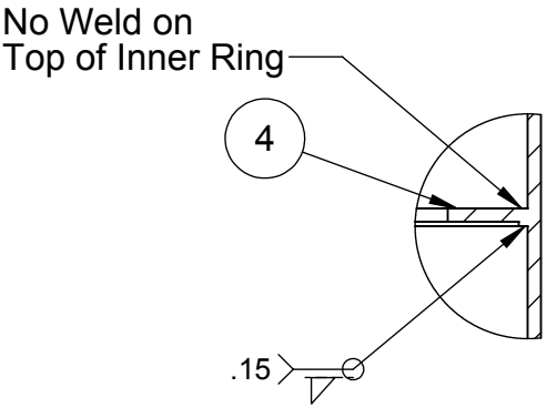
DETAIL E SCALE 1 : 3
