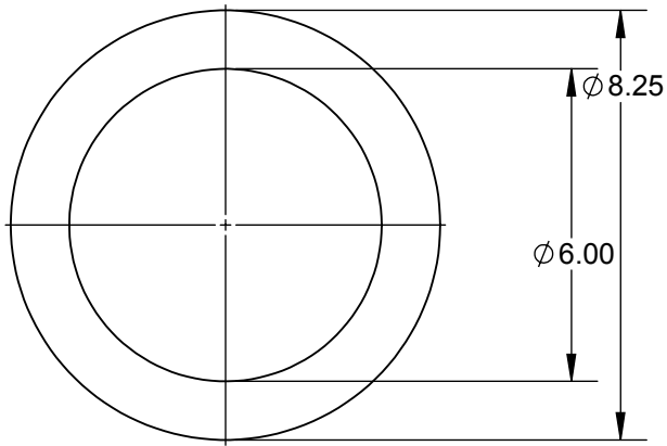
Inner Ring A36 Steel
