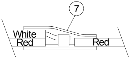
SPLICE DETAIL - 2 SPLICES SOLDER & HEAT SHRINK
