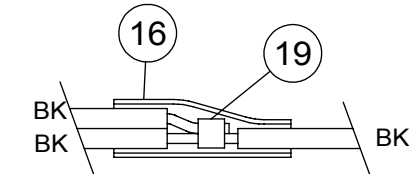
SPlice DETAIL - 6 SPLICES SOLDER & HEAT SHRINK
