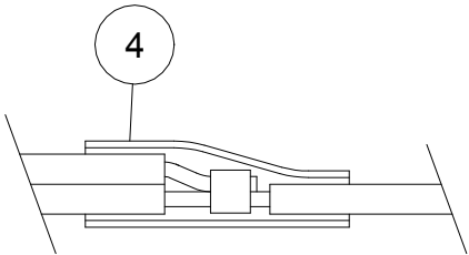
Splice Detail Solder & Heat Shrink 6 Splices
