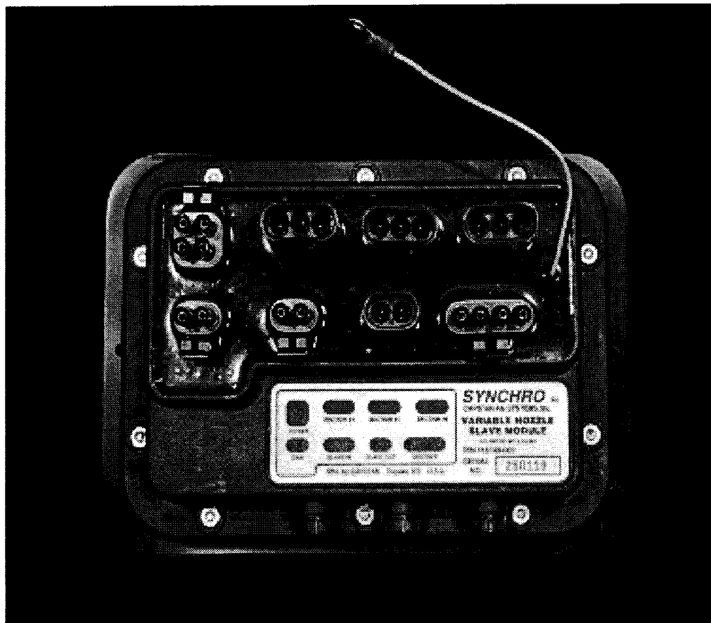
Figure 5. - Detailed connections and “pin-out” of the Synchro Slave Flow Control Module. This is the front view and the label is in the position we’ll call the “lower right” of the module.
