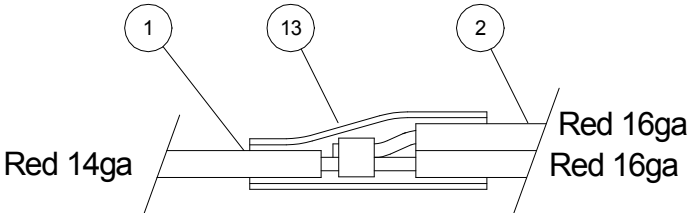
SPLICE DETAIL SOLDER & HEAT SHRINK NOTE 1
