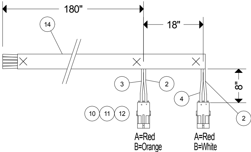
SPLICE DETAIL SOLDER & HEAT SHRINK NOTE 1
