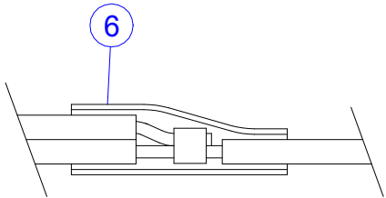
Splice Detail Solder & Heat Shrink 3 Splices
