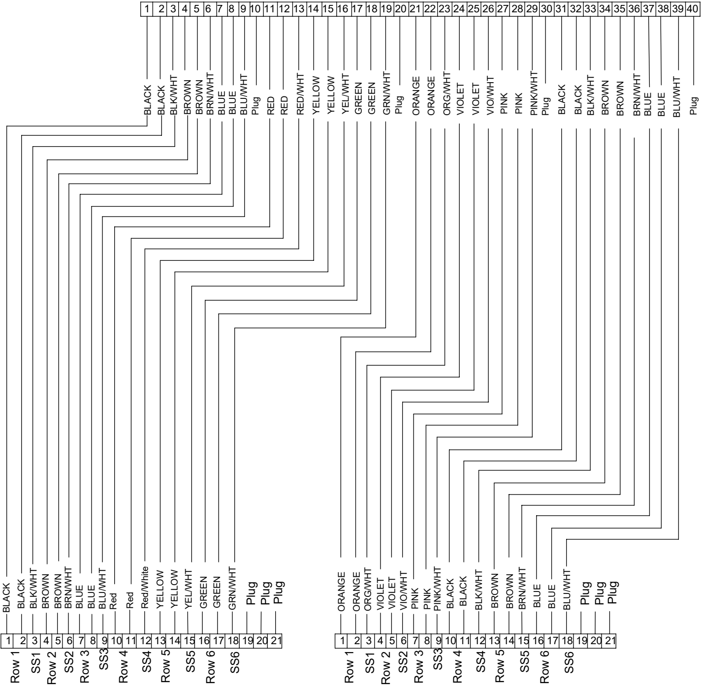
21 Pin HDP Receptical, #20 Contacts Receptical 1 Left Side
