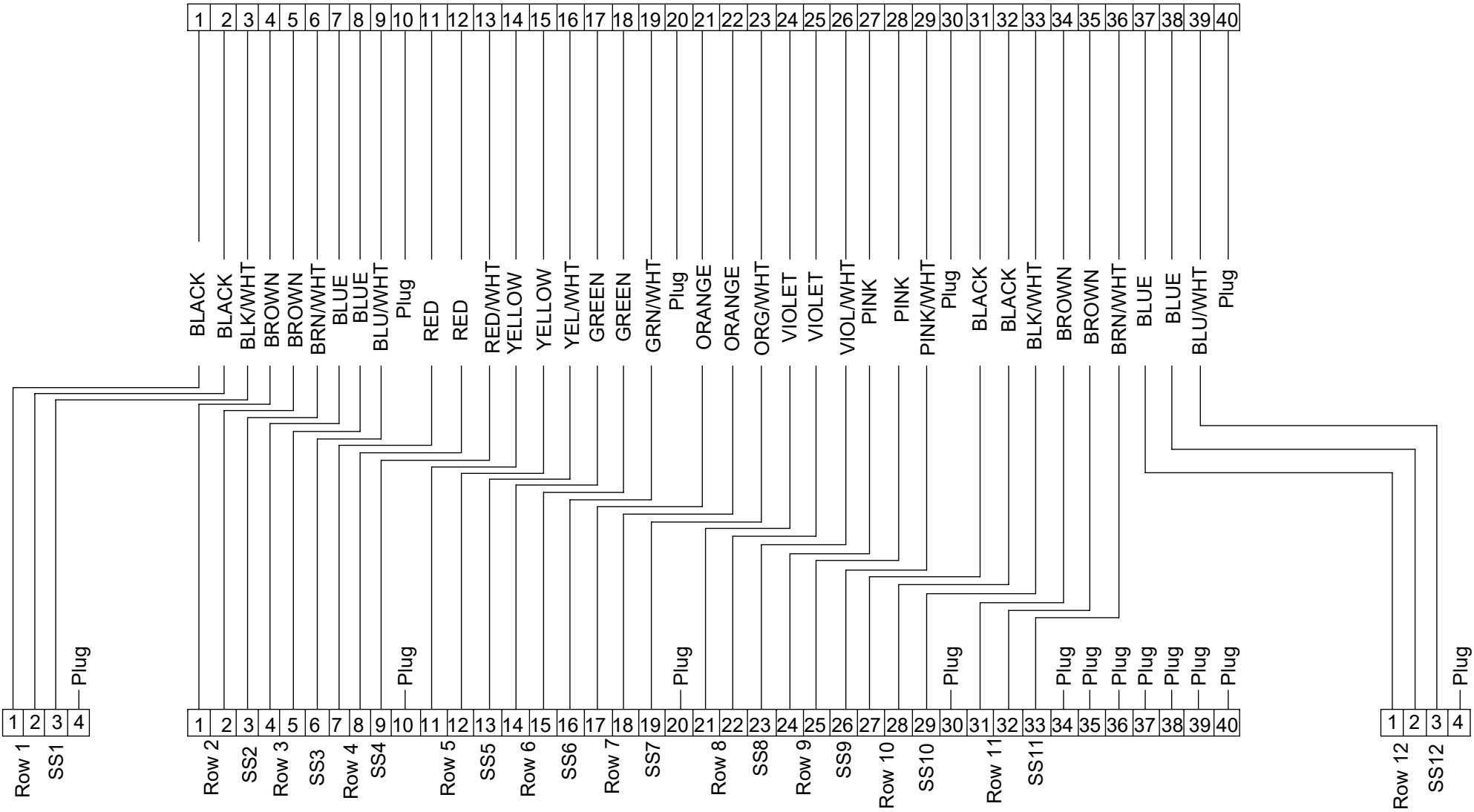
40 Pin DRC Plug, #20 Contacts (Controller)
