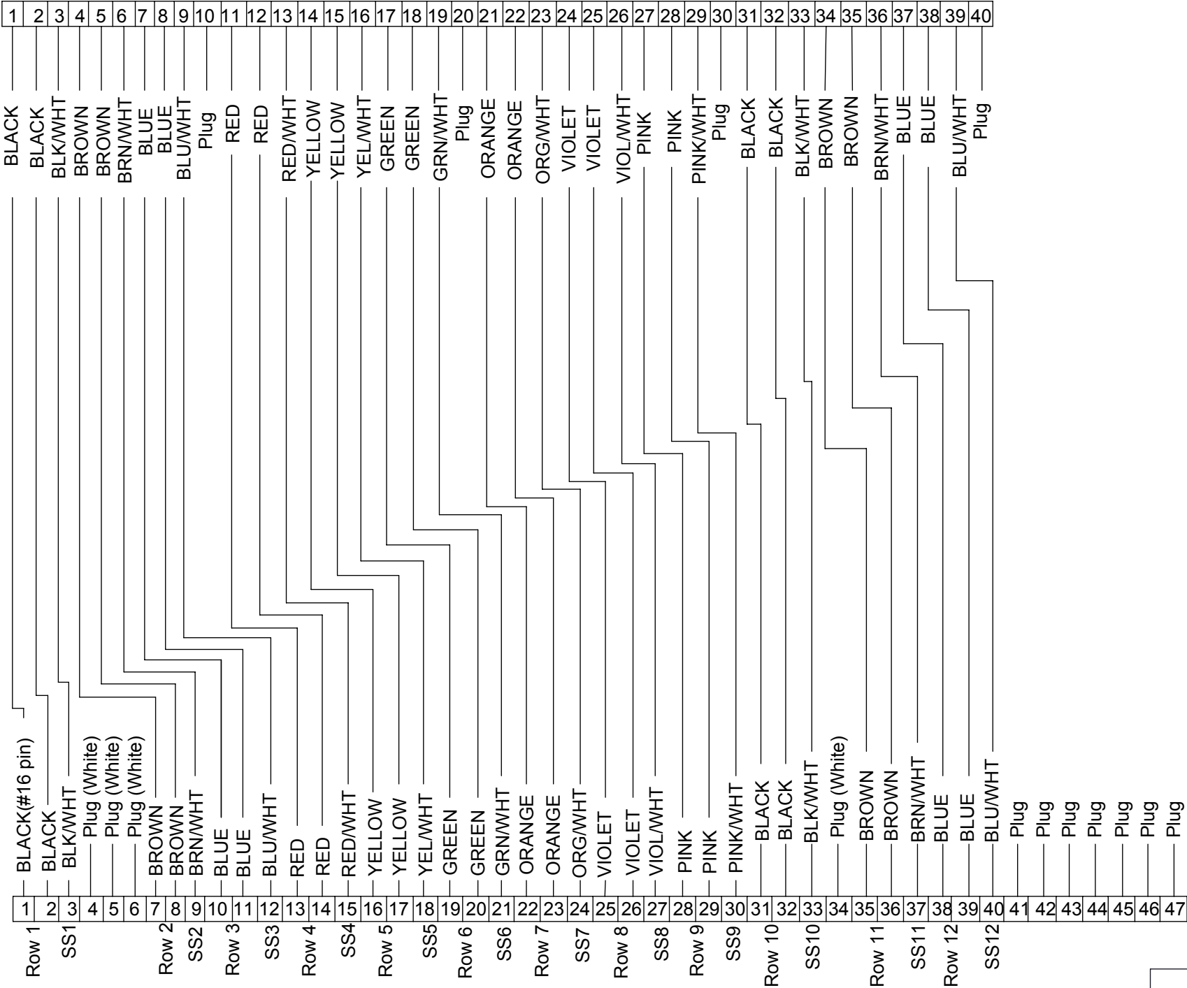
47 Pin HDP Plug, #20 Contacts
