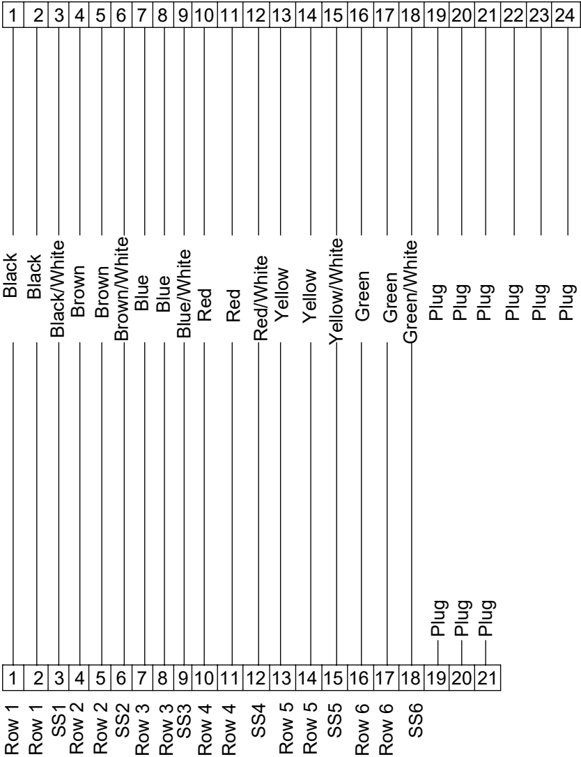
21 Pin HDP Plug, #20 Contacts
