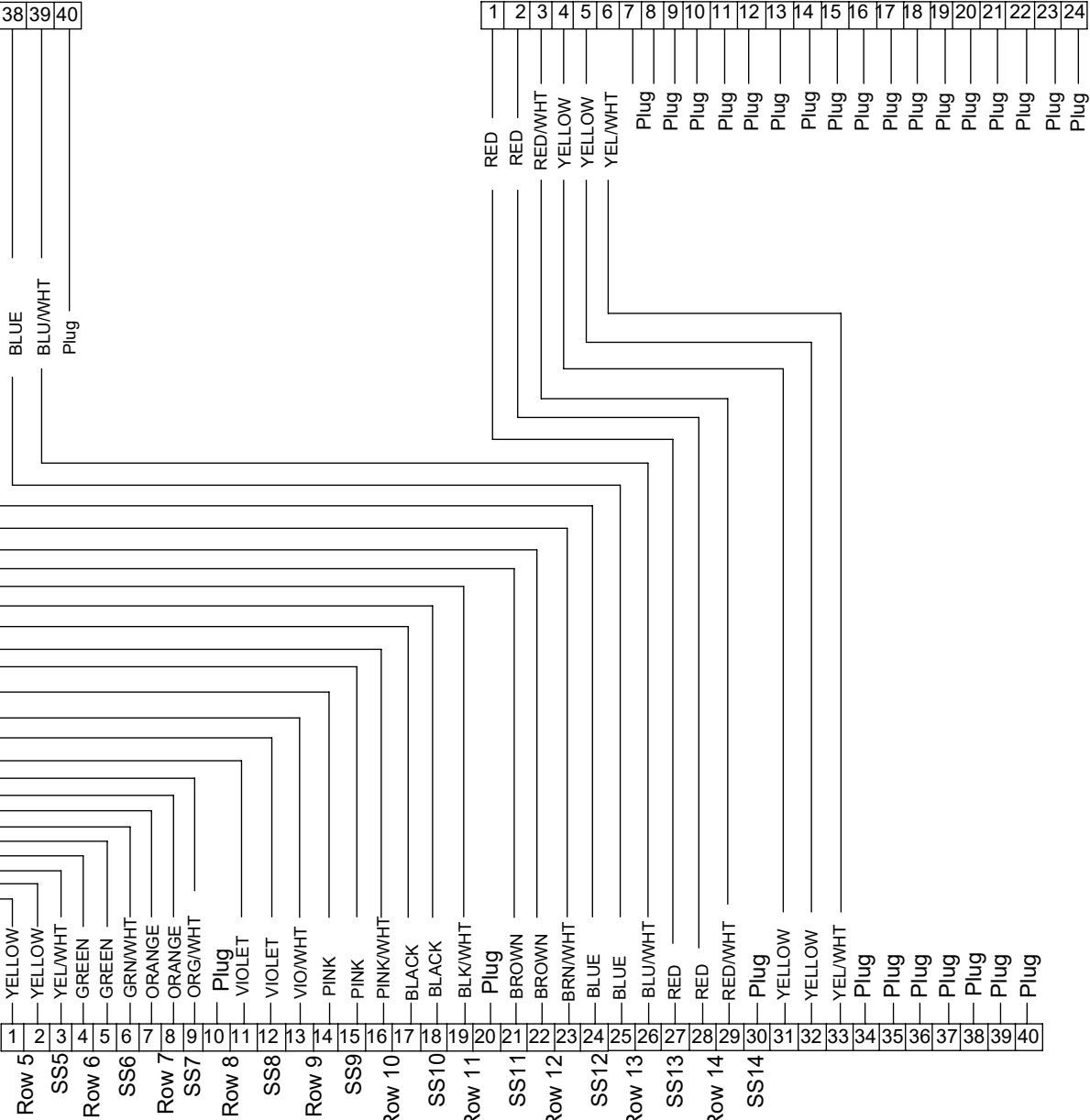
40 Pin DRC Receptical, #16 Contacts Receptical 2
