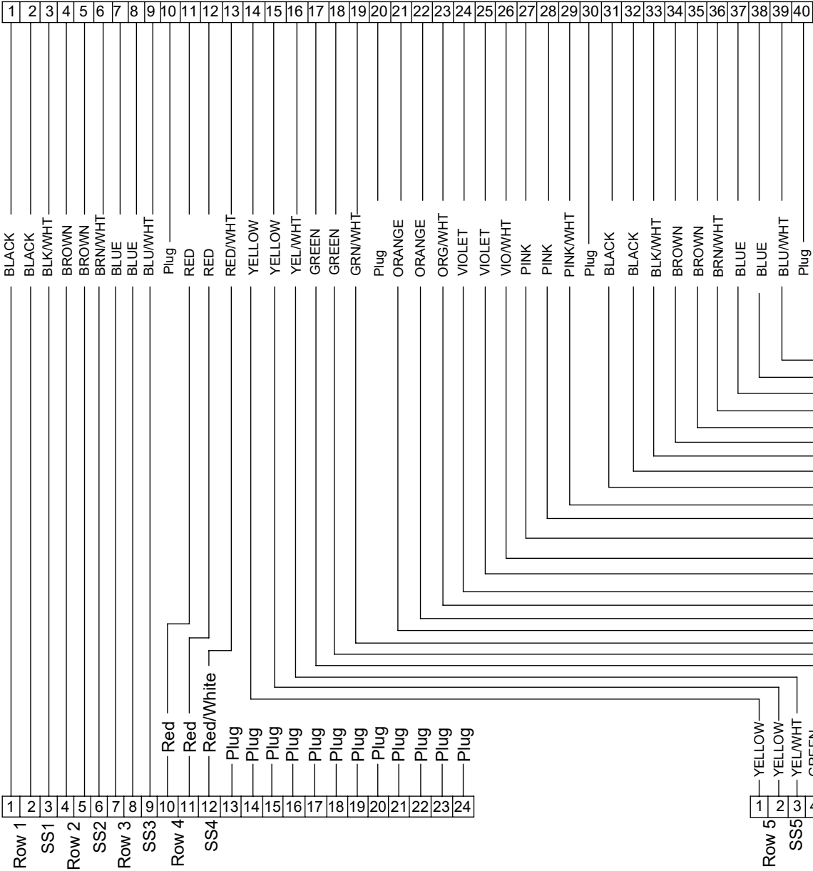
24 Pin DRC Receptical, #16 Contacts Receptical 1
