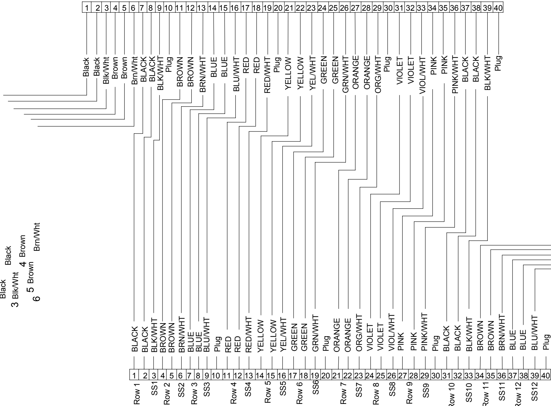
40 Pin DRC Receptical, #16 Contacts
