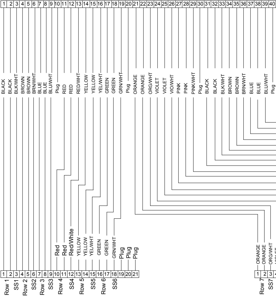
21 Pin HDP Receptical, #20 Contacts Receptical 1 Left Side
