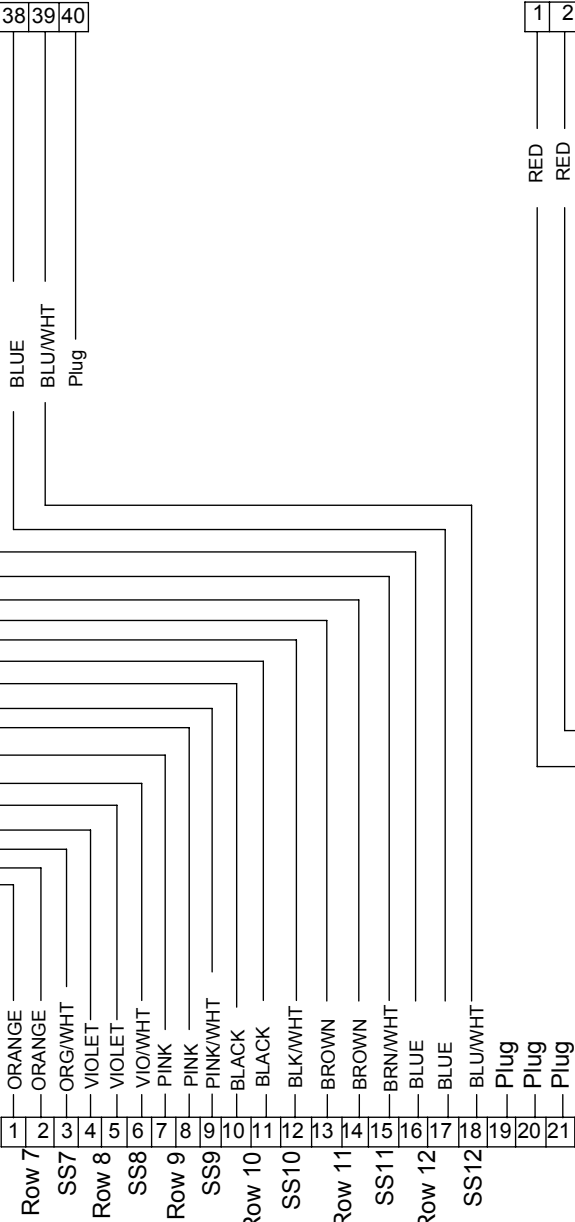
21 Pin HDP Receptical, #20 Contacts Receptical 2 Center
