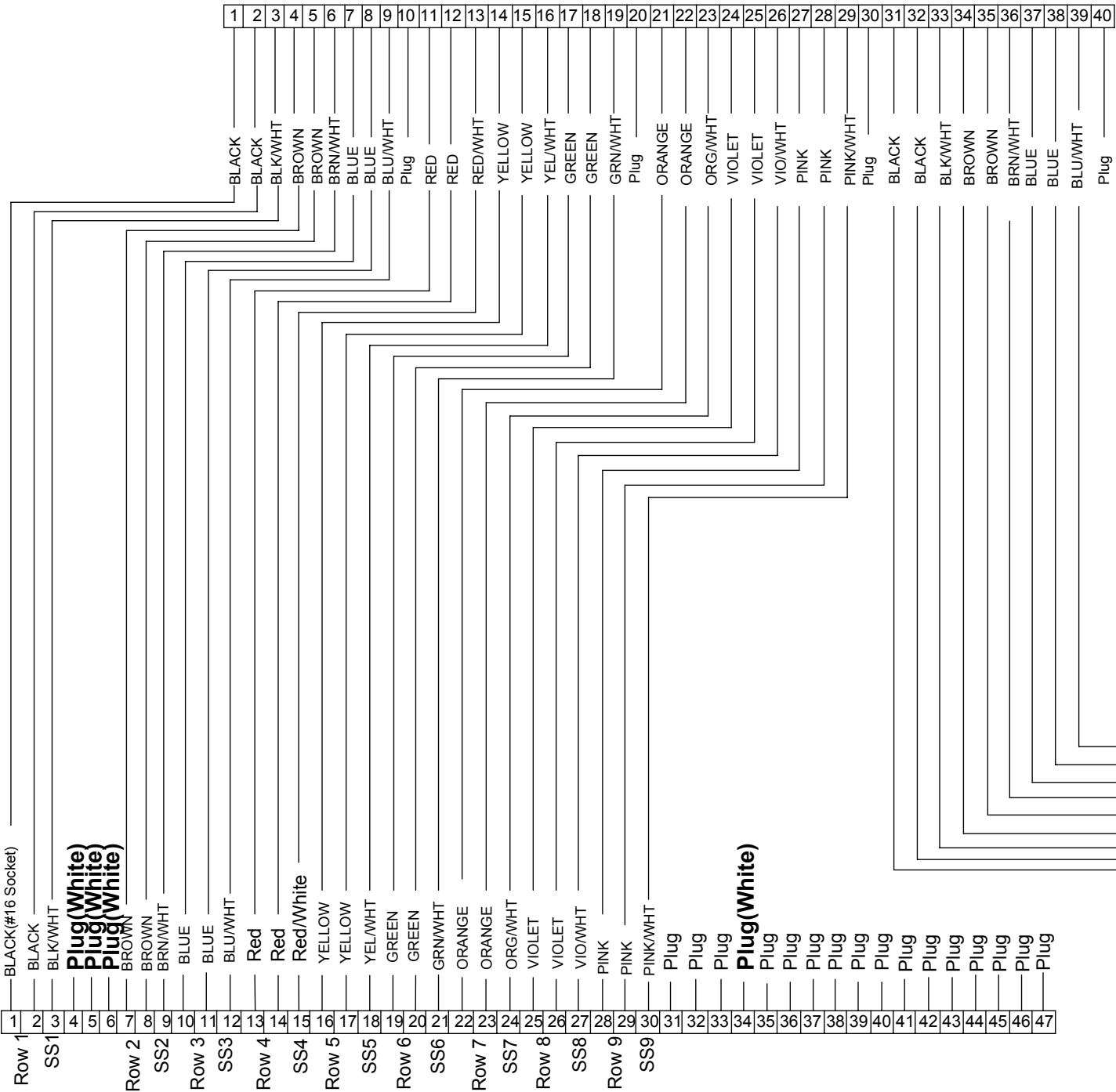
40 Pin DRC Plug, #20 Contacts
