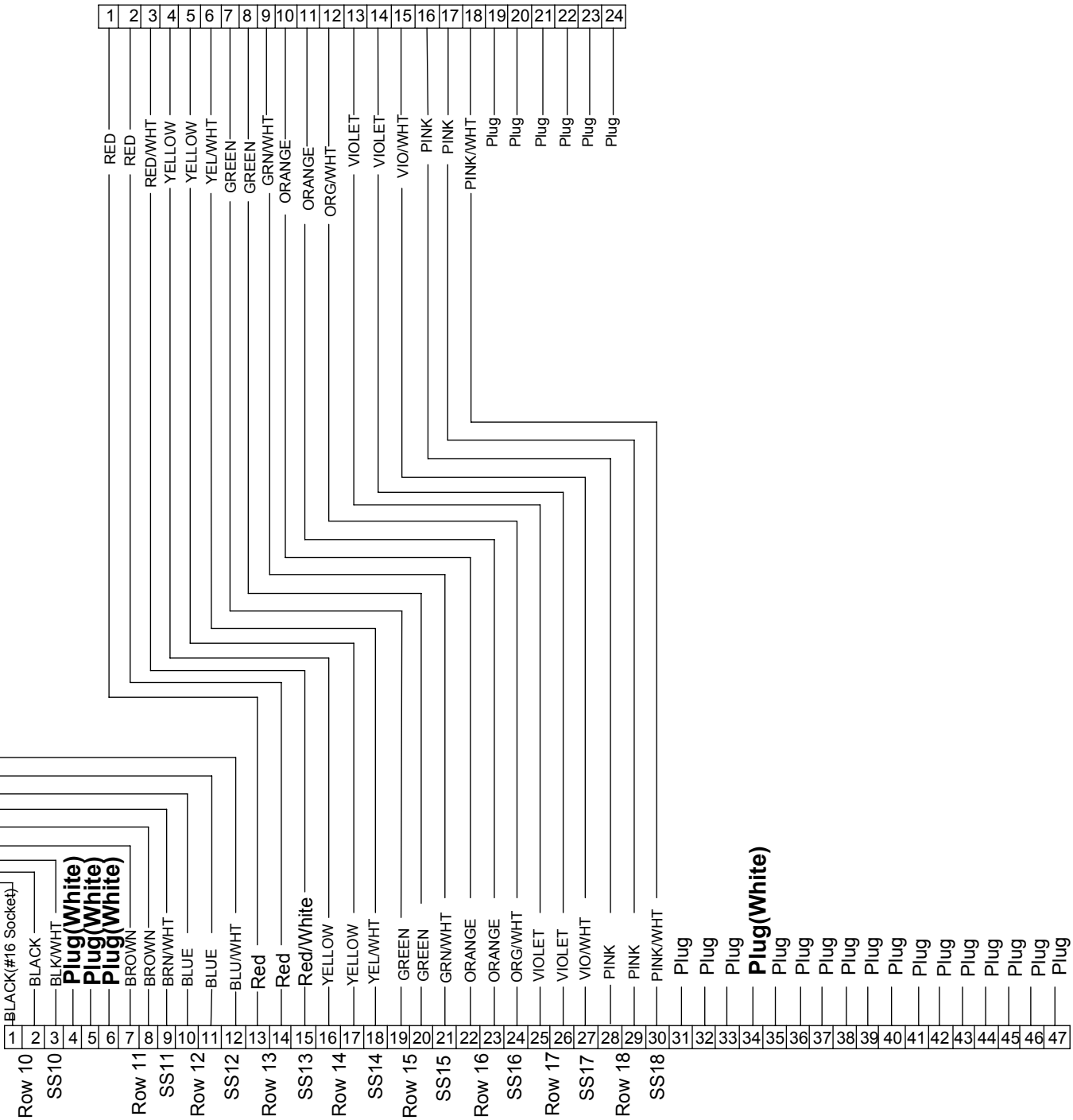
24 Pin DRC Plug, #20 Contacts
