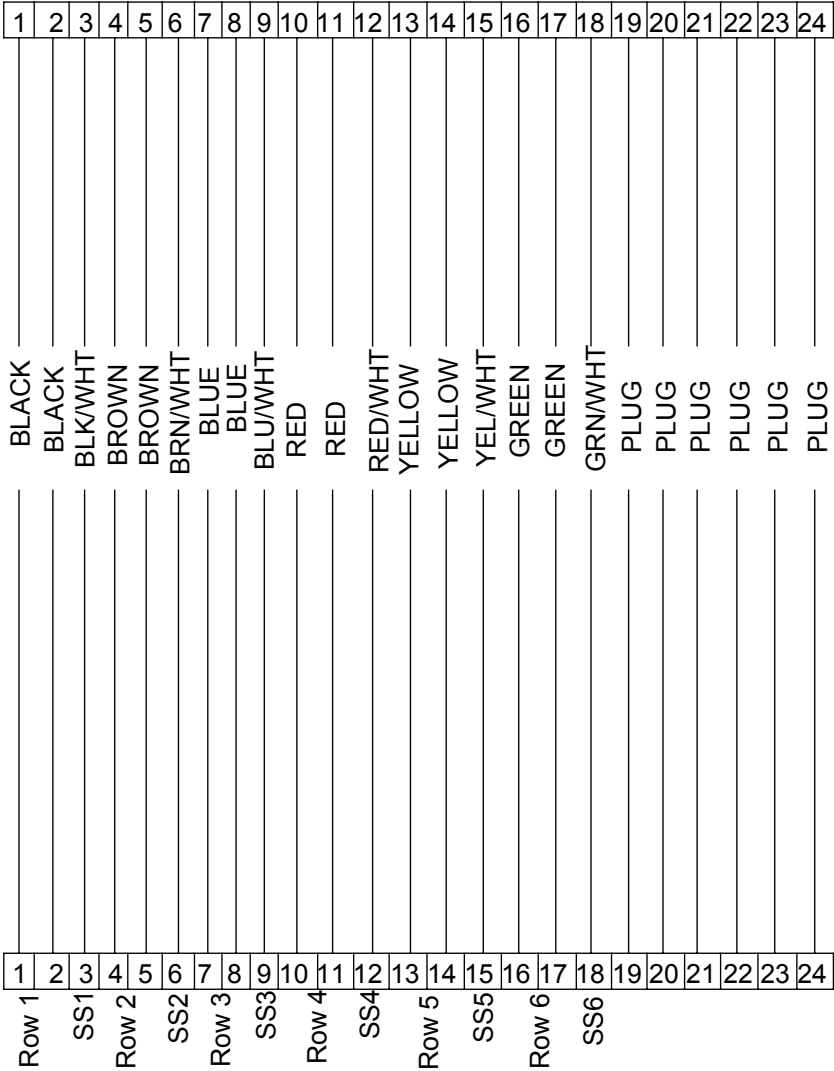
24 Pin DRC Receptical, #16 Contacts
