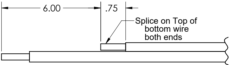
Splice Detail, -4 Pls
