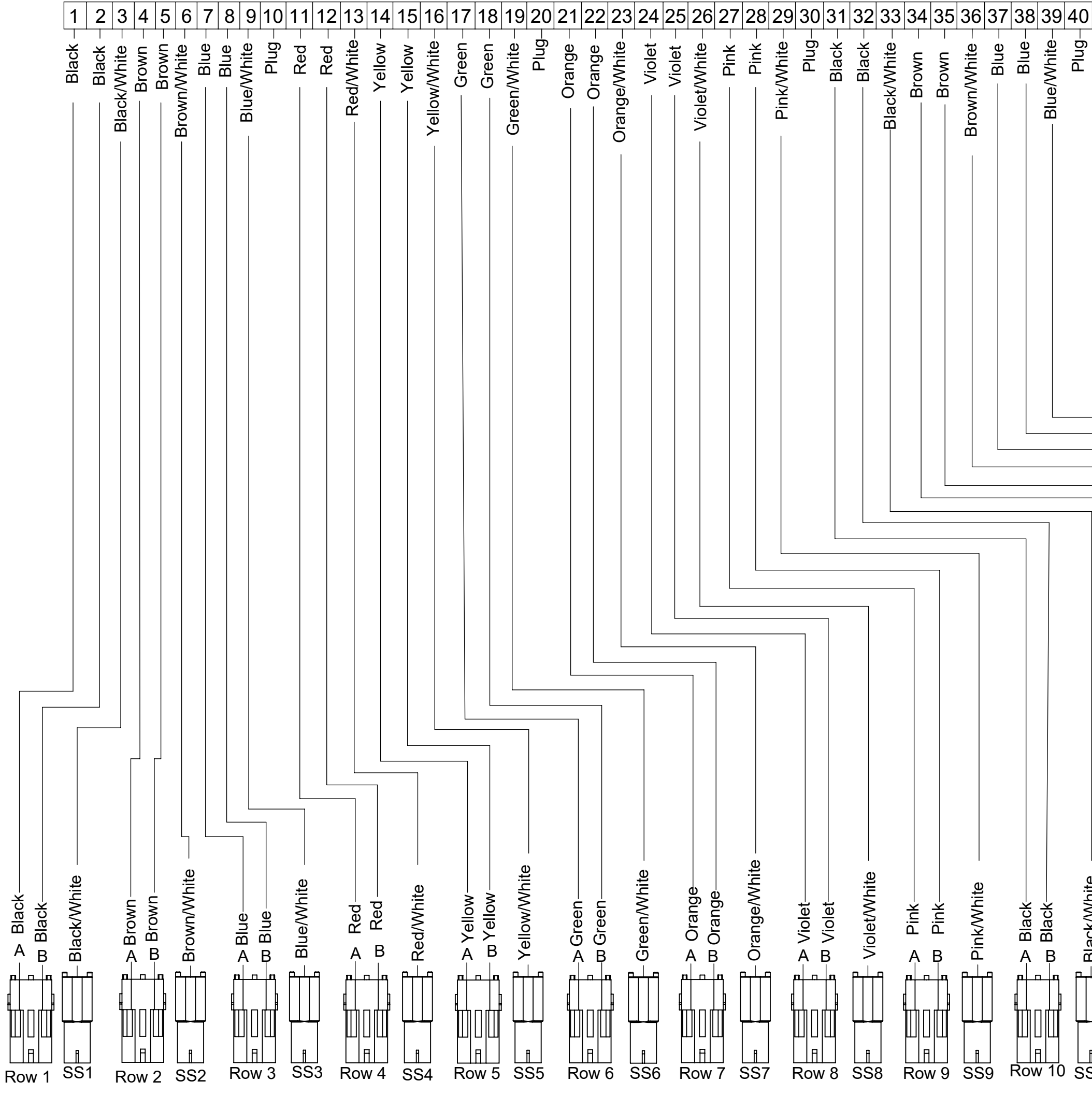
40 Pin DRC Plug, #16 Contacts
