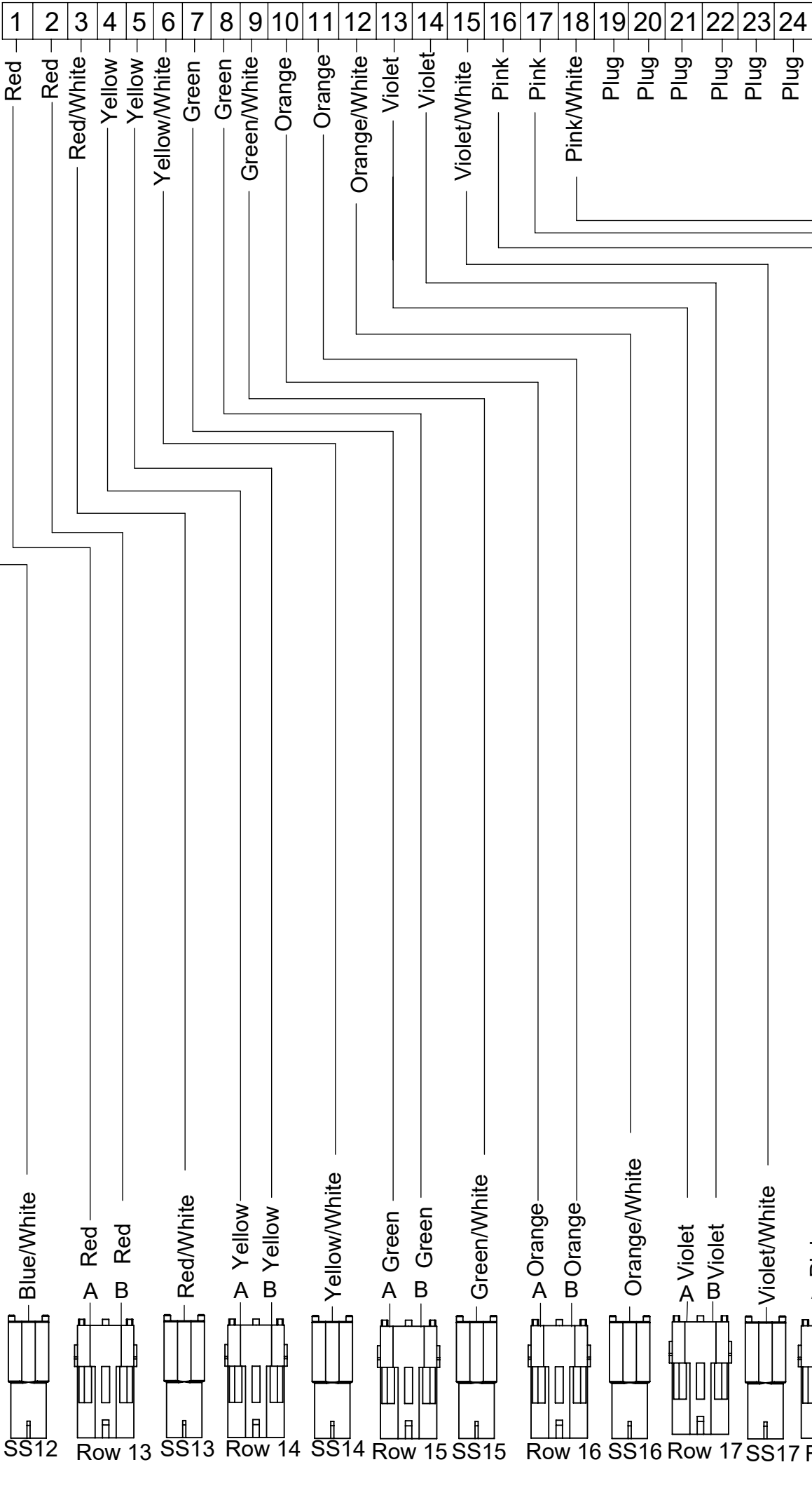
24 Pin DRC Plug, #16 Contacts
