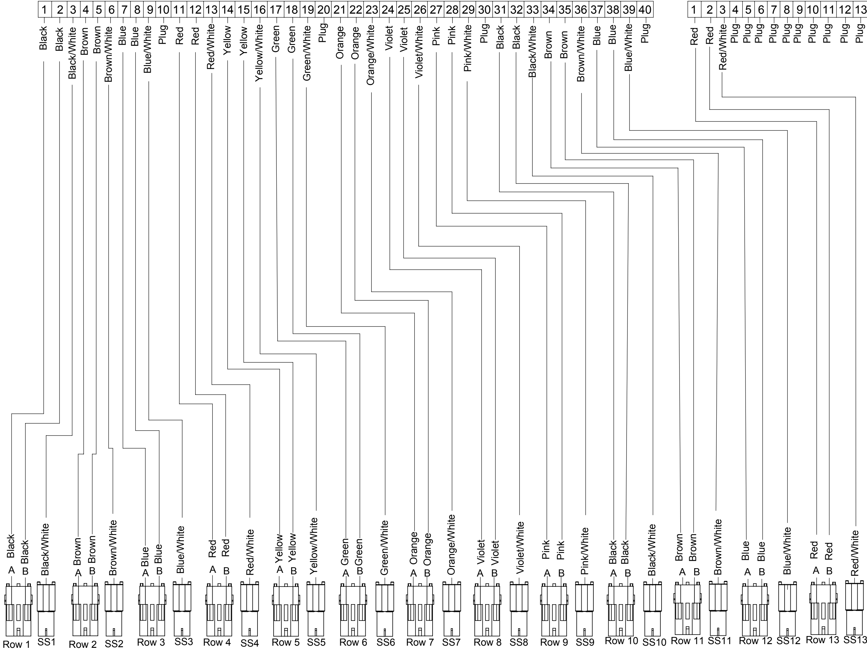
40 Pin DRC Plug, #16 Contacts
