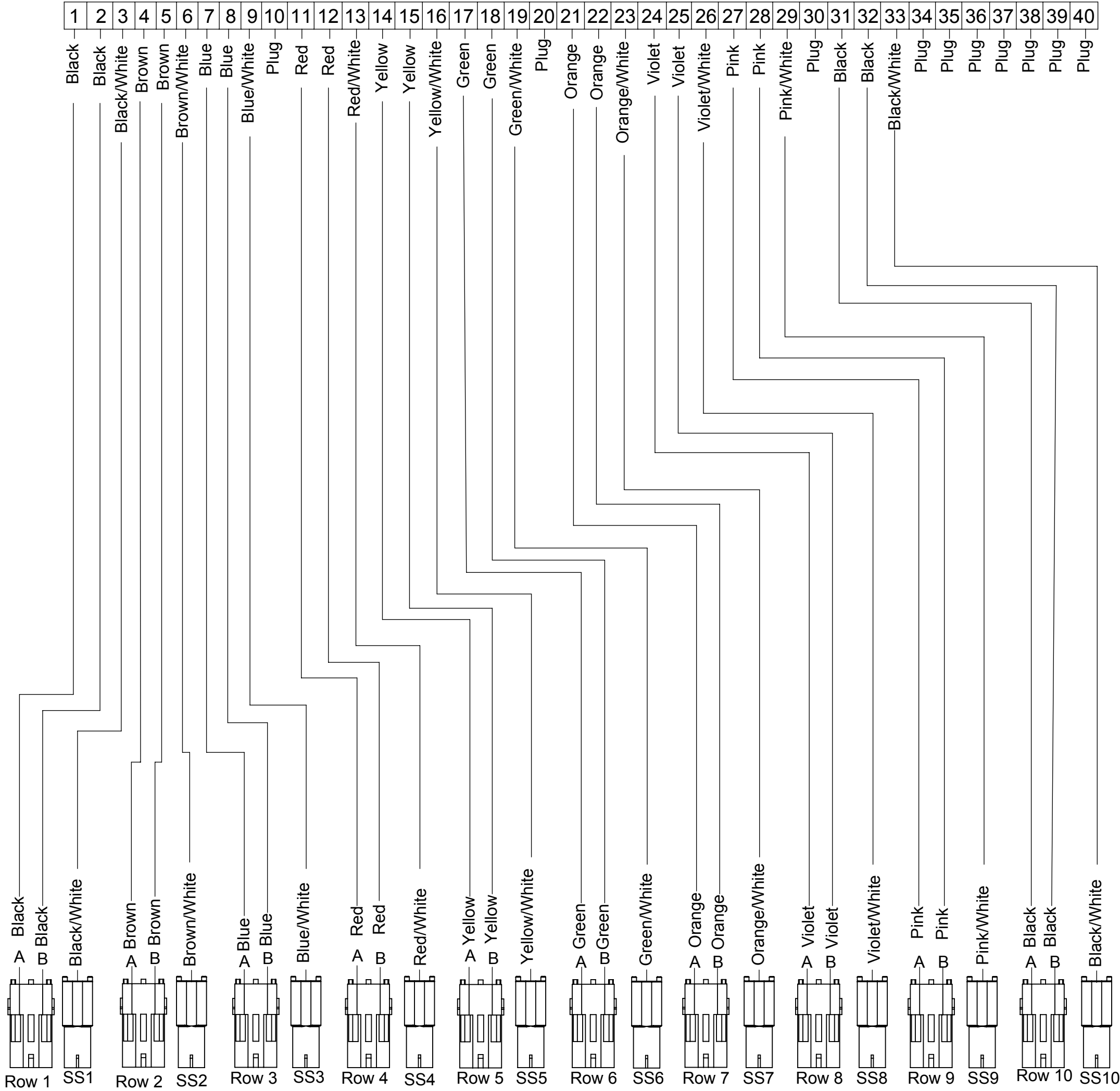
40 Pin DRC Plug, #16 Contacts
