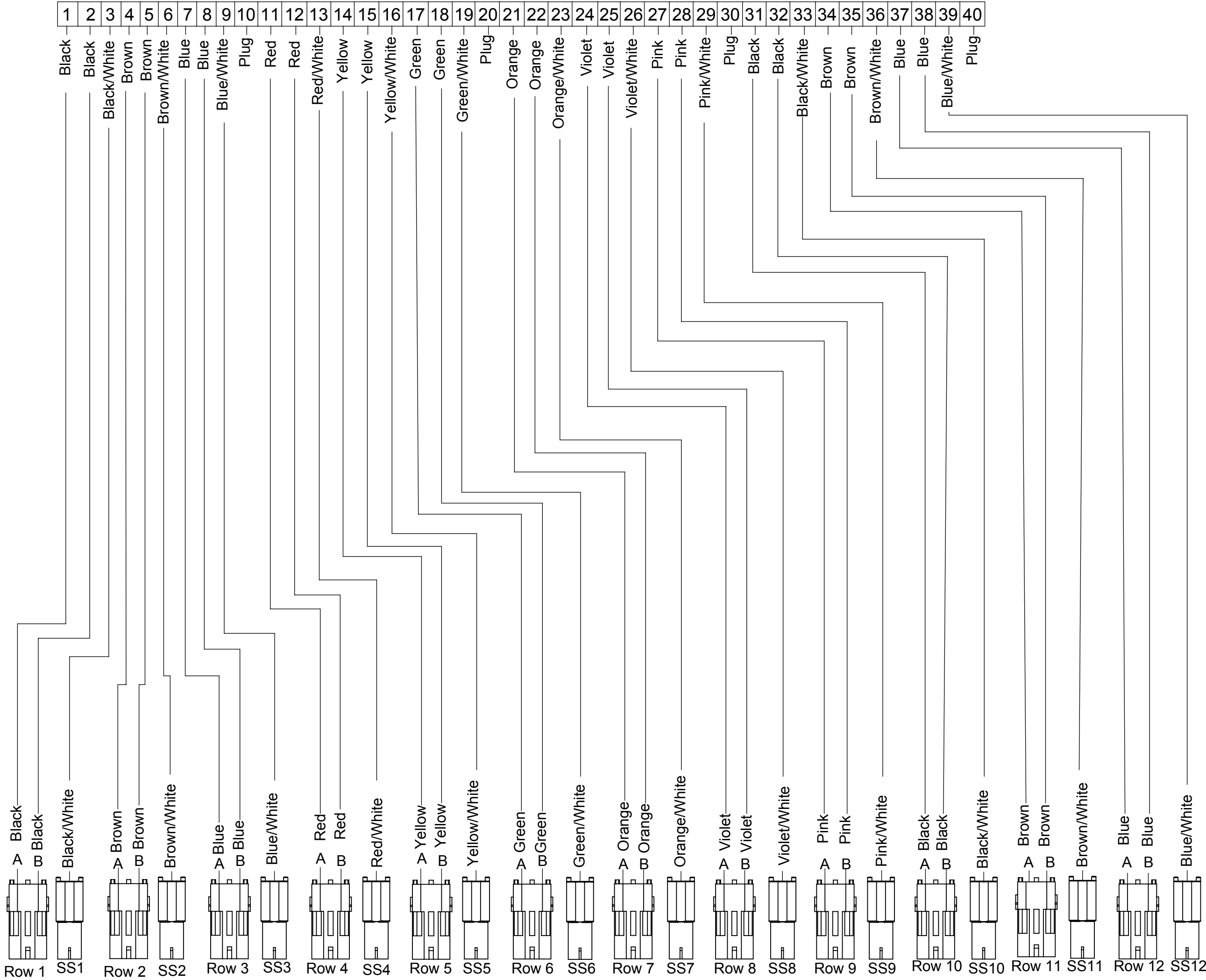
40 Pin DRC Plug, #16 Contacts
