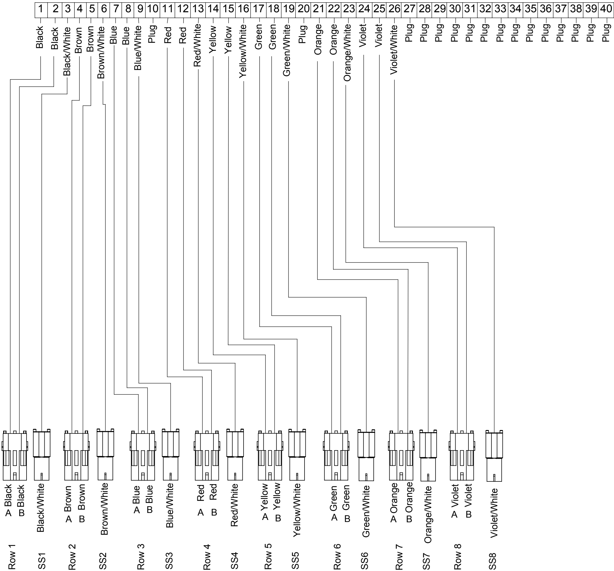
40 Pin DRC Plug, #16 Contacts
