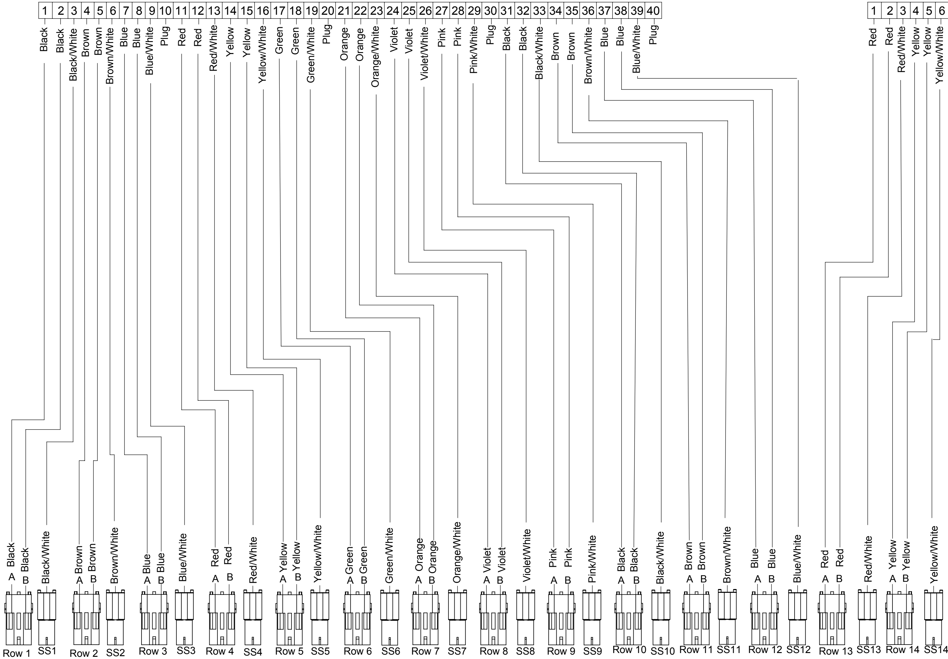
40 Pin DRC Plug, #16 Contacts
