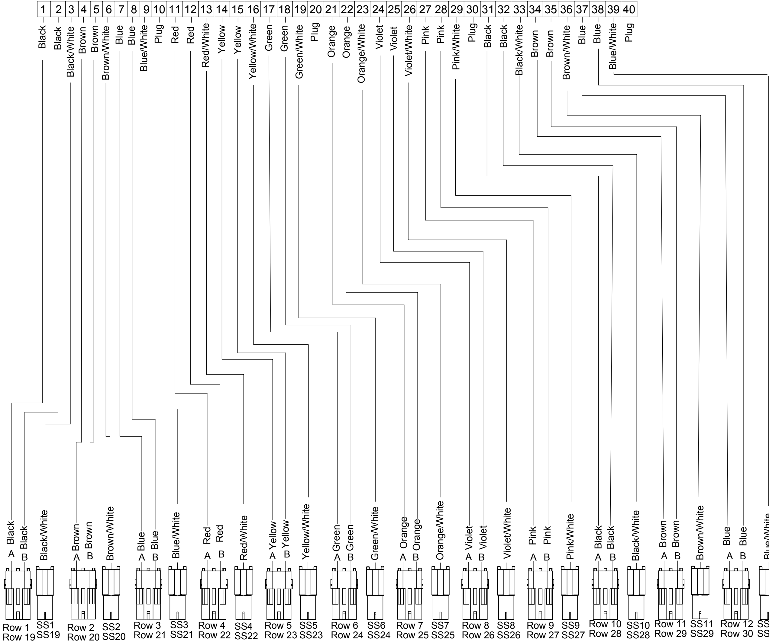
40 Pin DRC Plug, #16 Contacts
