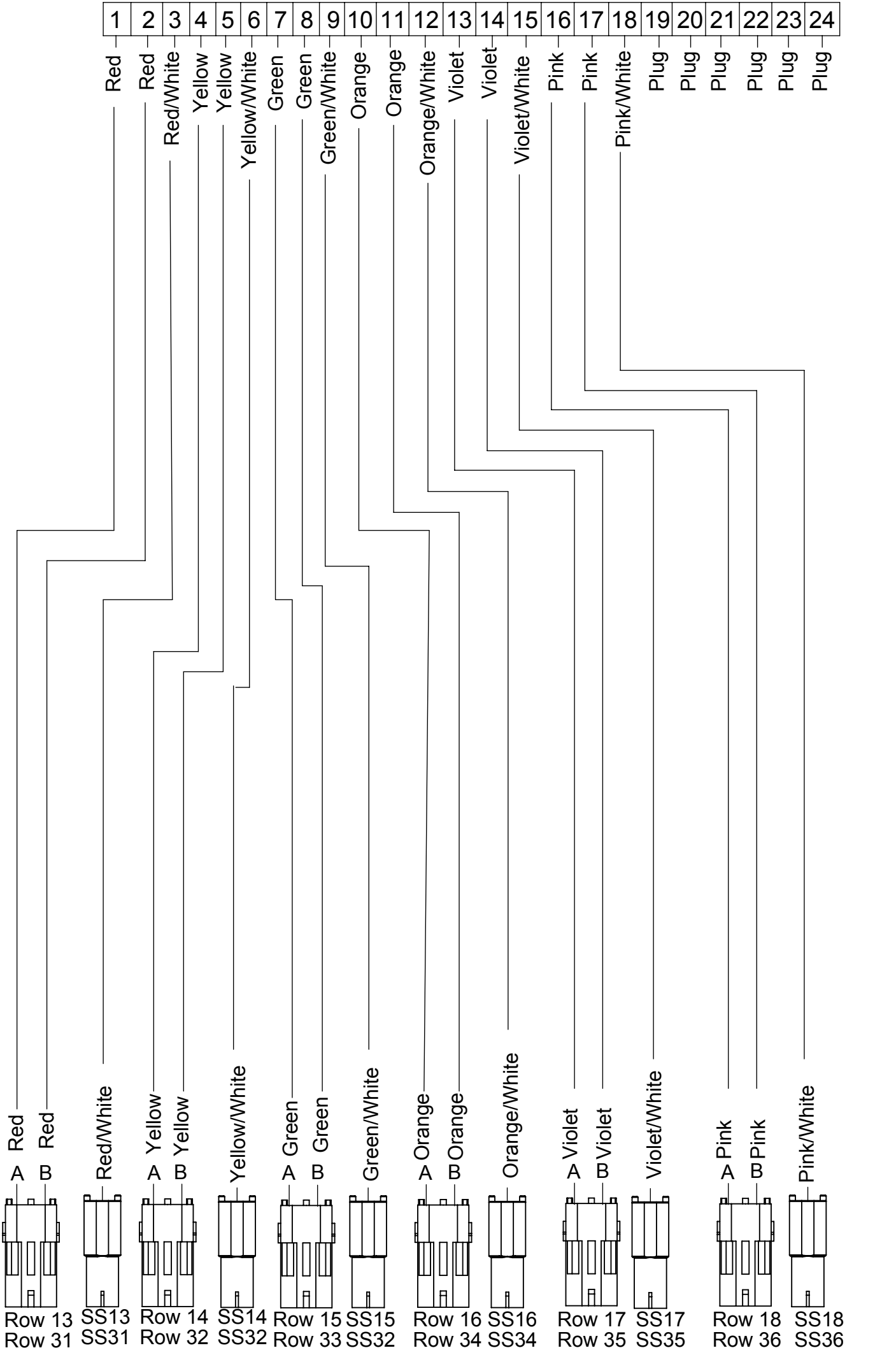
24 Pin DRC Plug, #16 Contacts
